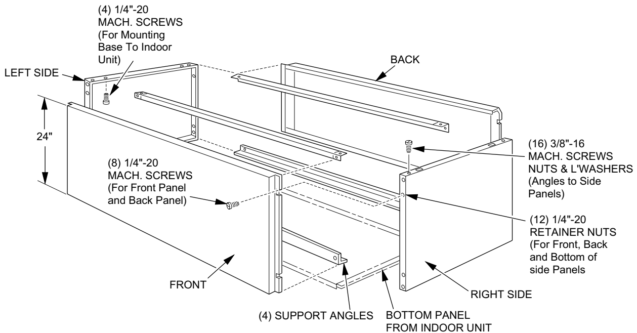
FIGURE 3 : BASE ACCESSORY MODEL 1BS0452
