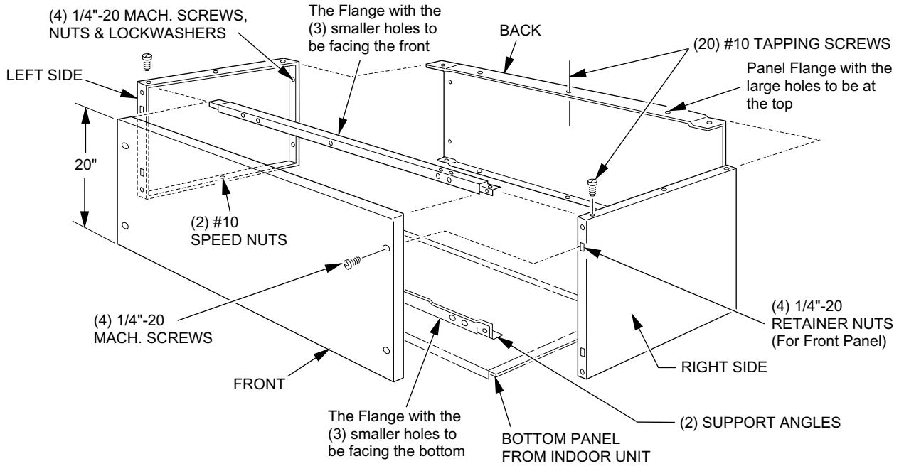
FIGURE 2 : BASE ACCESSORY MODELS 1BS0450 AND 1BS0451
