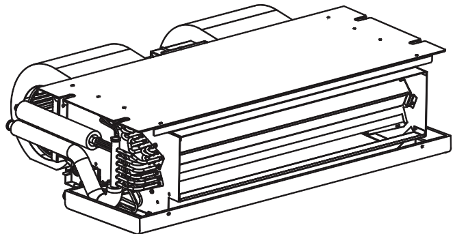
FMU4P - Uncased Horizontal Fan Coil
