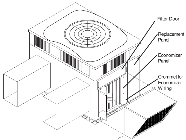
Horizontal Economizer
