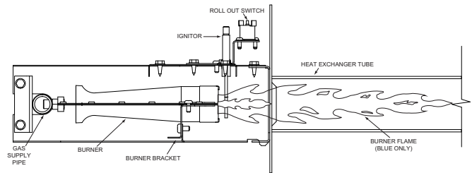
Figure 23: Typical Flame
