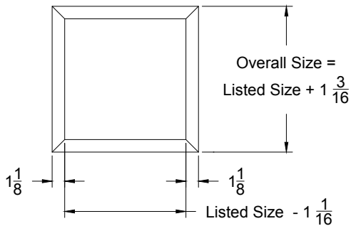
Face View (Models TBPf and STBPf)
