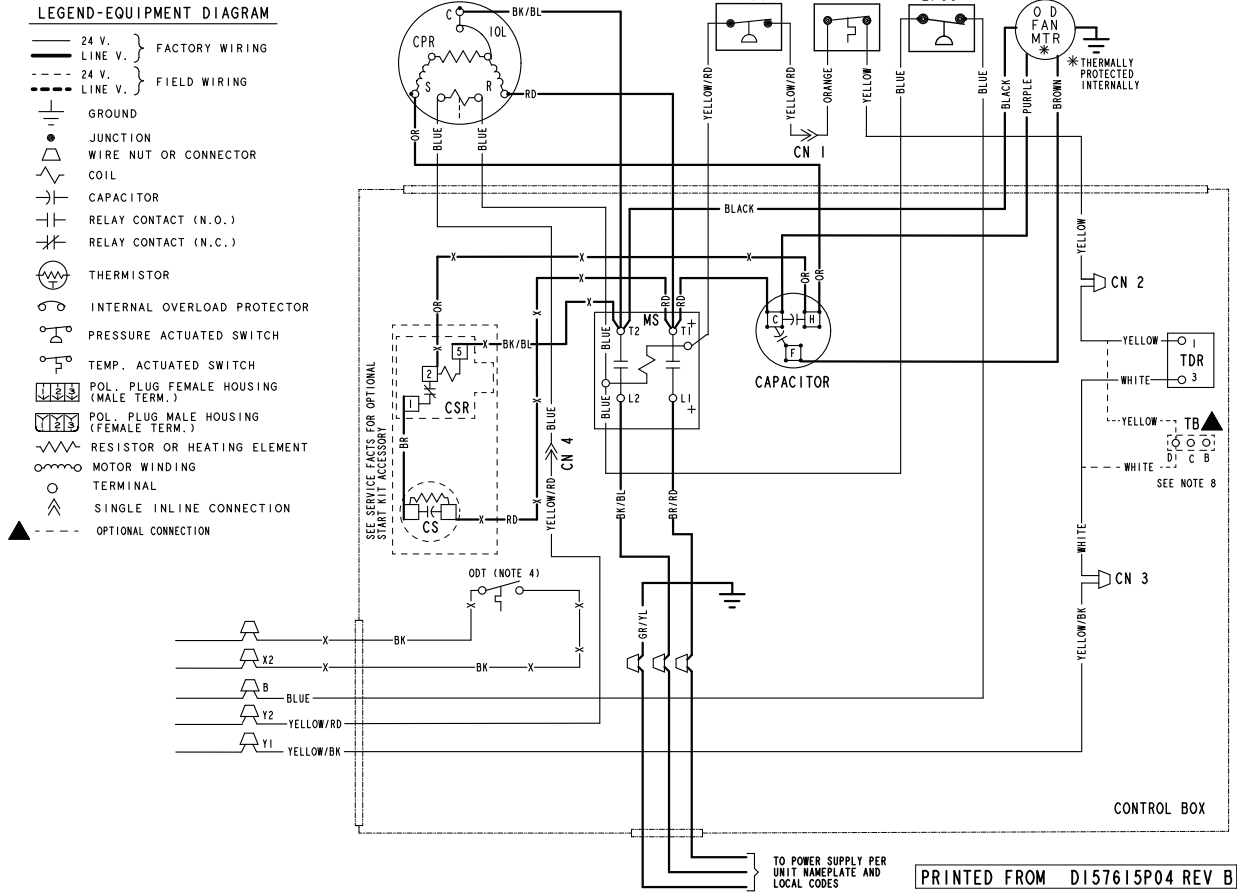
Figure 2. 024N & 036N Models
