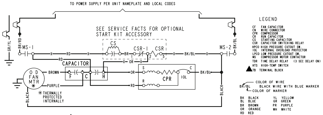
Figure 1. 024N & 036N Models
