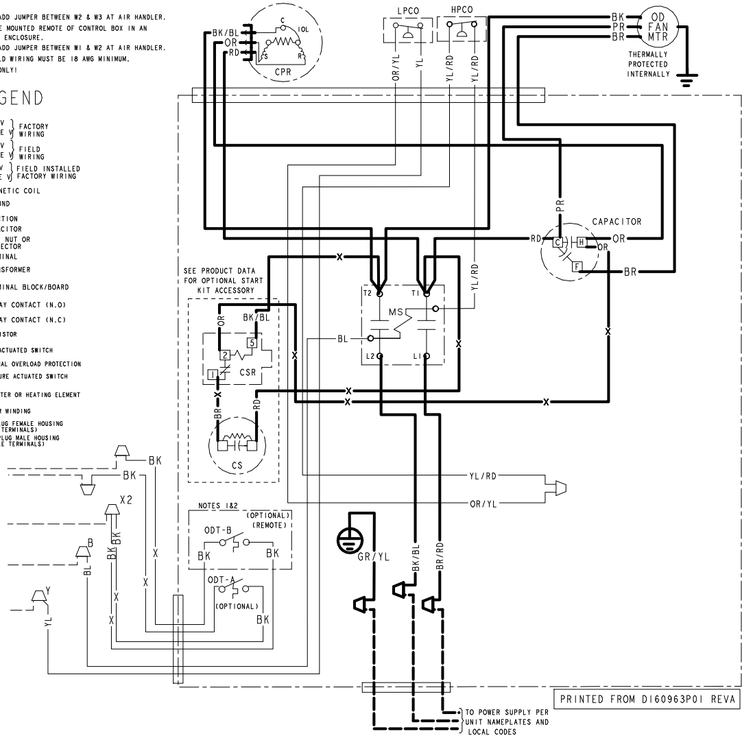
Figure 14. 060J & 060K Models
