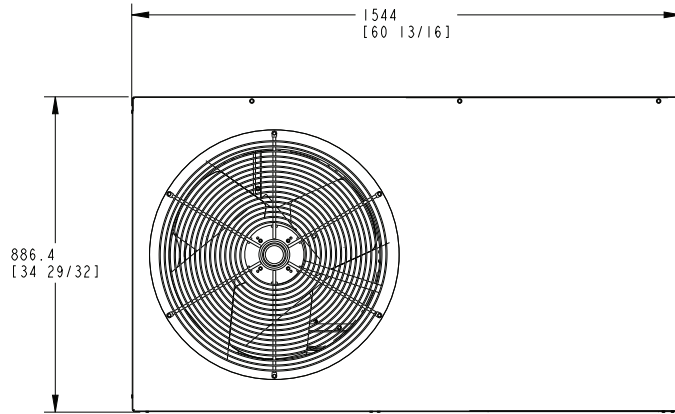
Figure 1. OUTLINE DRAWING
