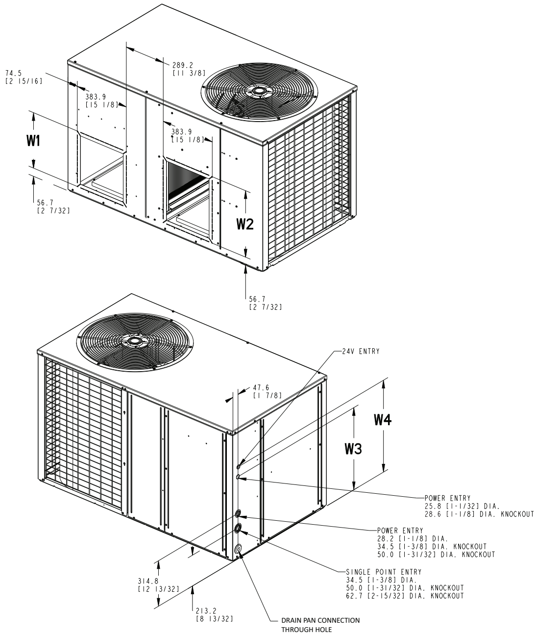
Figure 2. OUTLINE DRAWING
