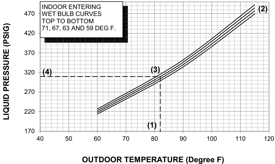
Figure 18. 3 Ton AC (X36 Models) 4TXCB004CC3HCB Cooling with Thermal Expansion Valve
