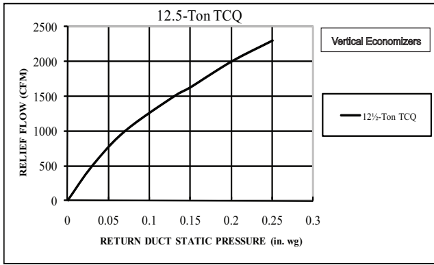
Fig. 22 - Relief Flow
