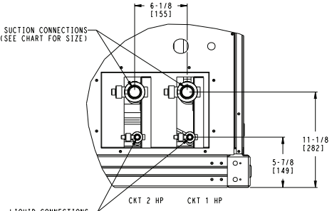
DETAIL A (NOTE POSITION OF CKT 1)
