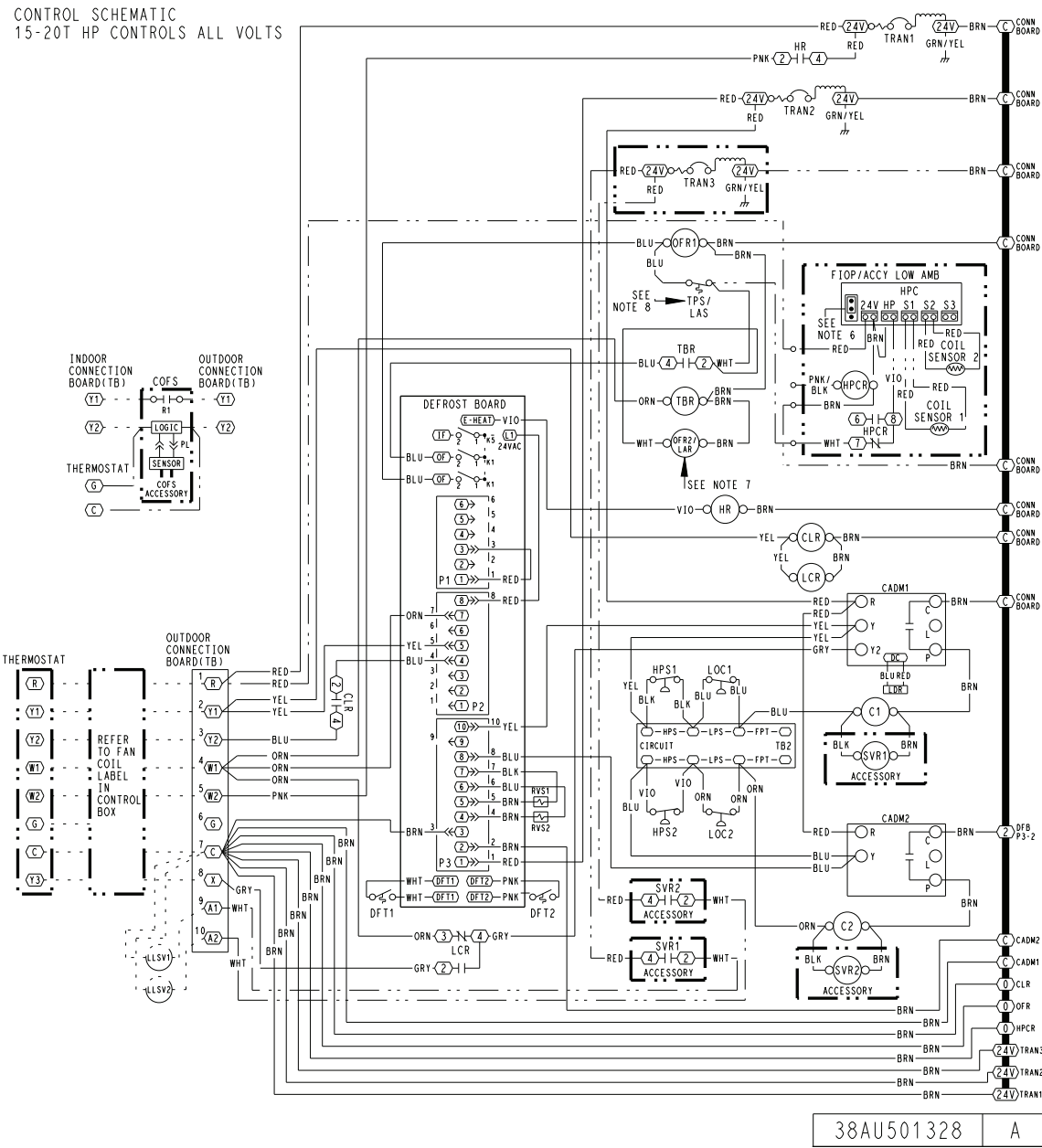
575J*16/25 Control Schematic
