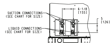
RIGHT SIDE VIEW (FOR 569JD SYSTEMS)
