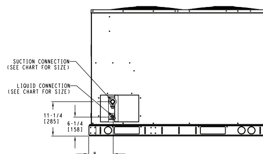
RIGHT SIDE VIEW (FOR 569JA AND 575JA SYSTEMS)
