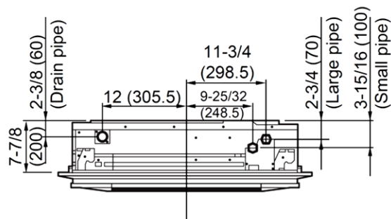
Side view (Slender setting)
