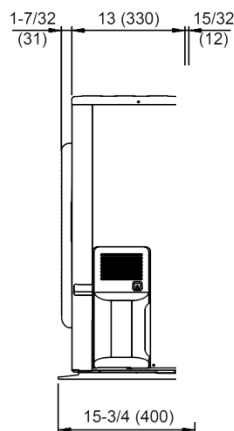
Side view (Standard setting)
