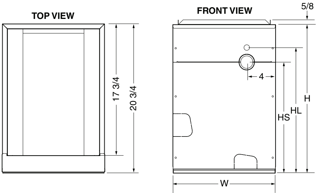
Figure 1. C74 Coil Dimensions (with TXV)
