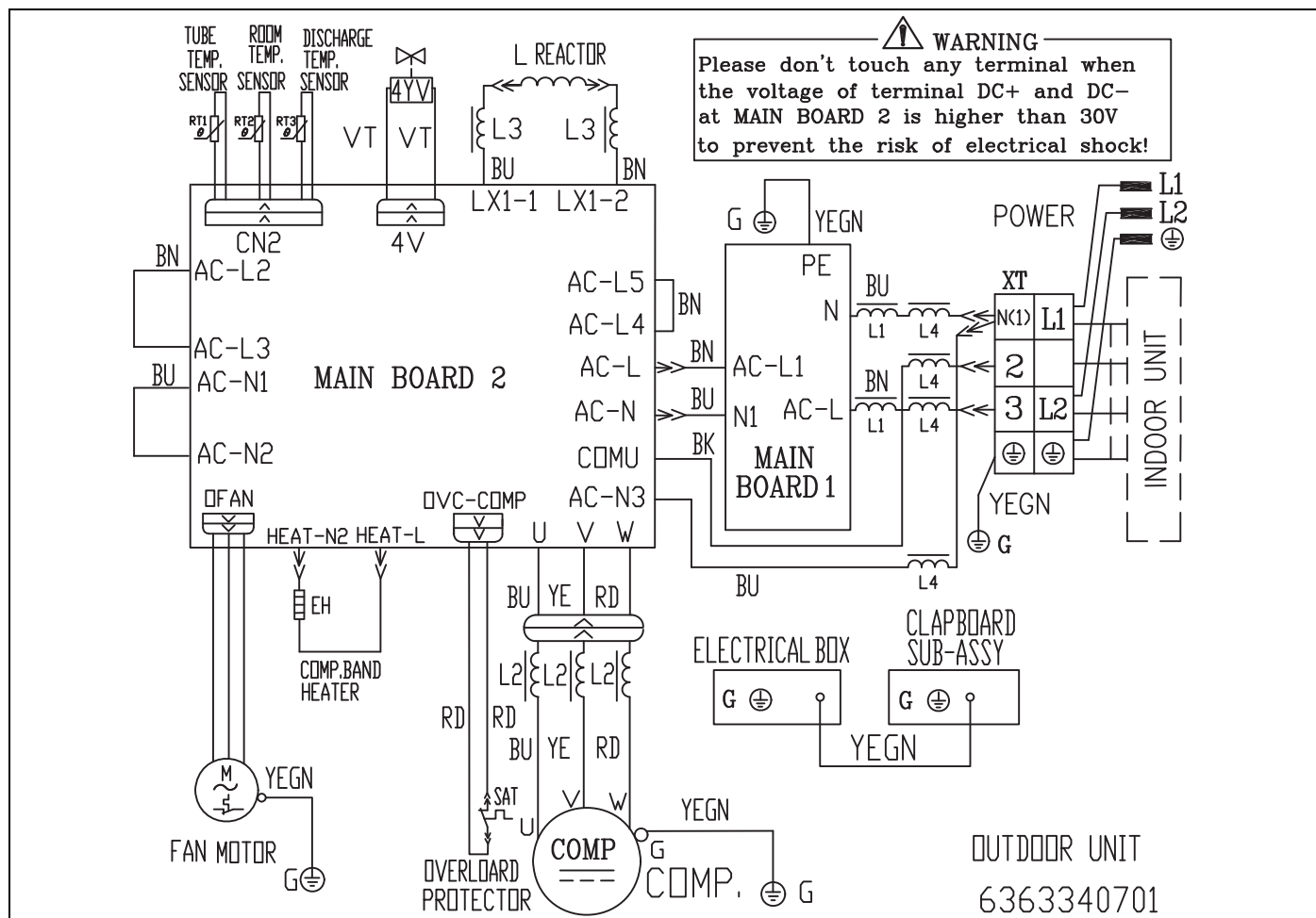
09K &amp; 12K Outdoor Heat Pumps
