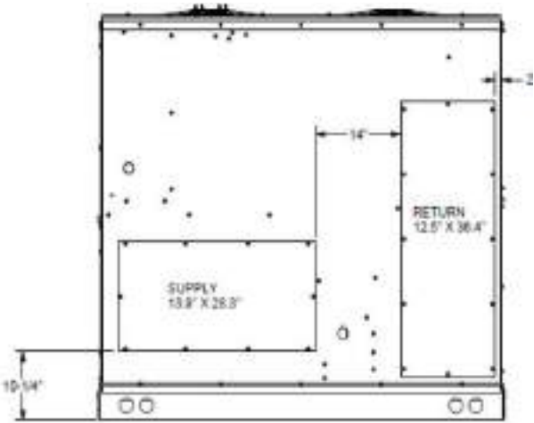
HORIZONTAL DISCHARGE
