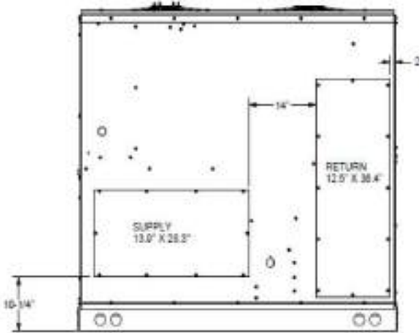
HORIZONTAL DISCHARGE
