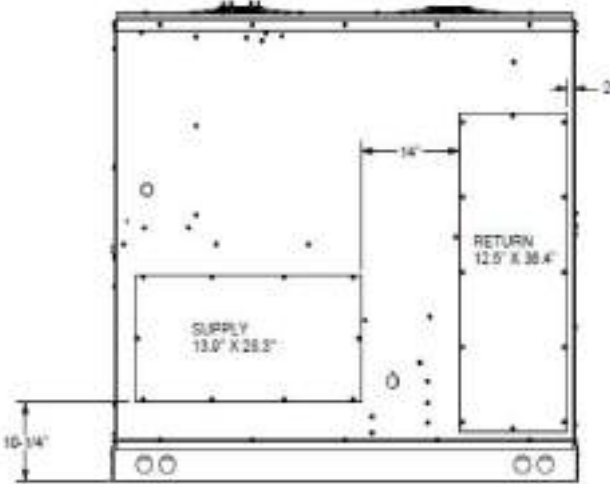
HORIZONTAL DISCHARGE
