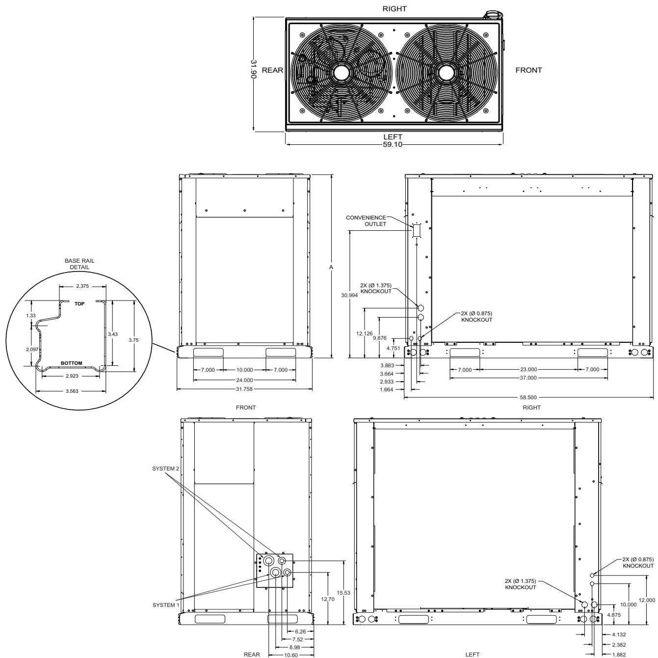
Unit dimensions PE090, PC120, YE090, YC/YD120, YC/YD150
