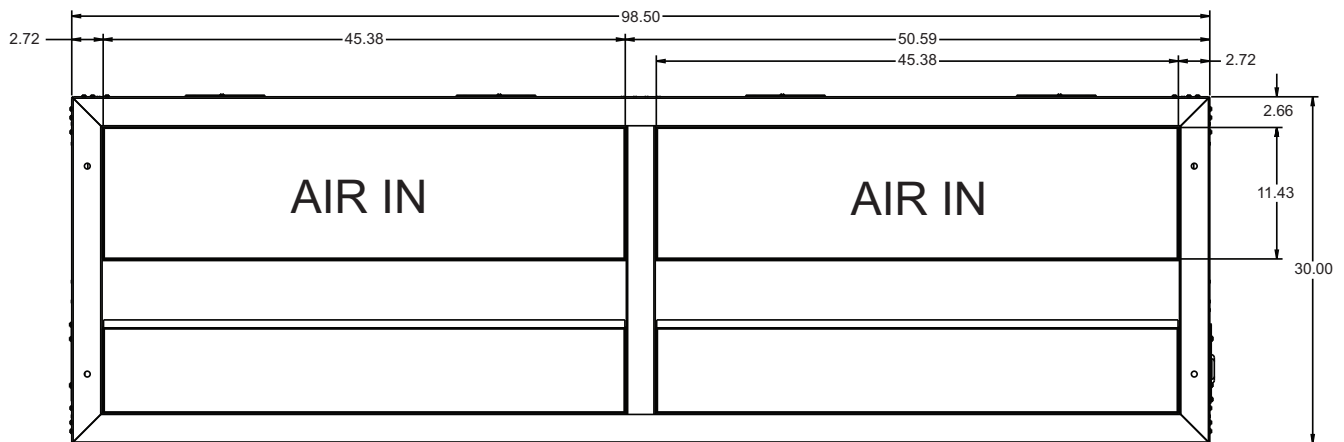
Bottom view
