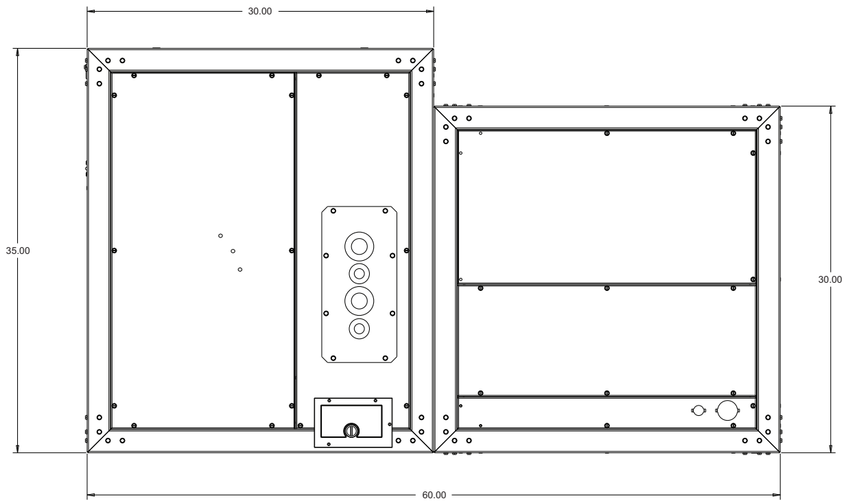
Horizontal configuration
