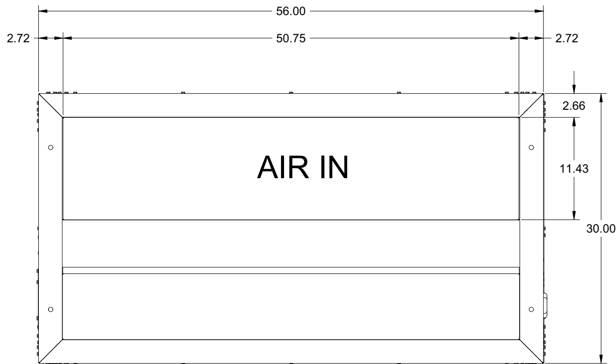
Horizontal configuration
