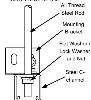
MOUNTING DETAIL
