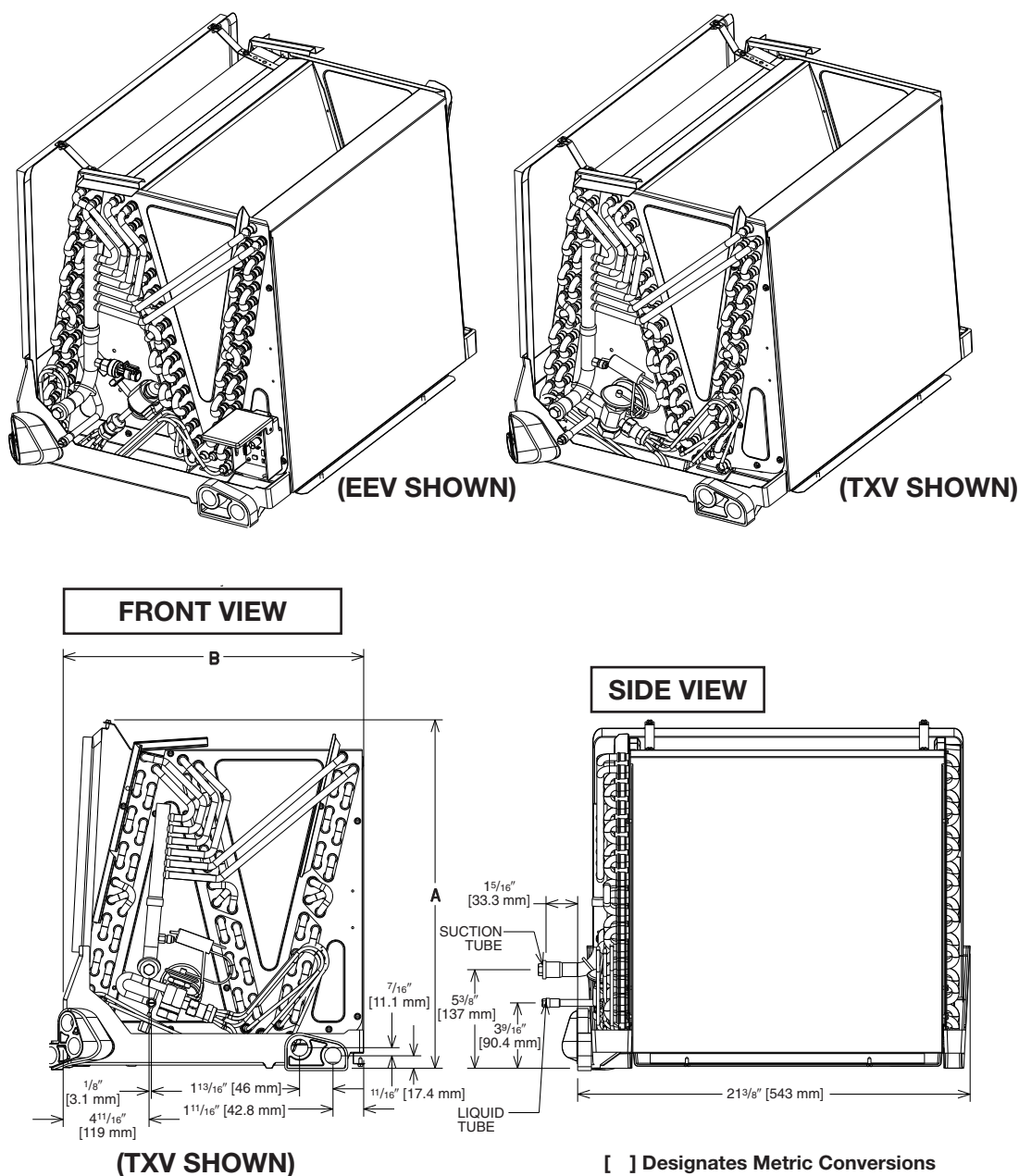
FIGURE 1: DIMENSIONS UNCASSED
