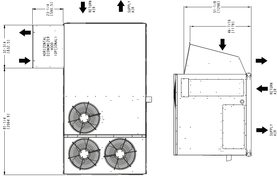
UNIT DIMENSIONAL DRAWING - UNIT SIZE RGS180 (cont)
