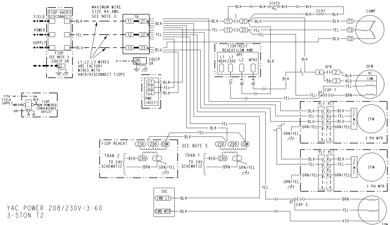
TYPICAL RGW036-060 POWER WIRING DIAGRAM, 208-230/3/60 UNIT SHOWN
