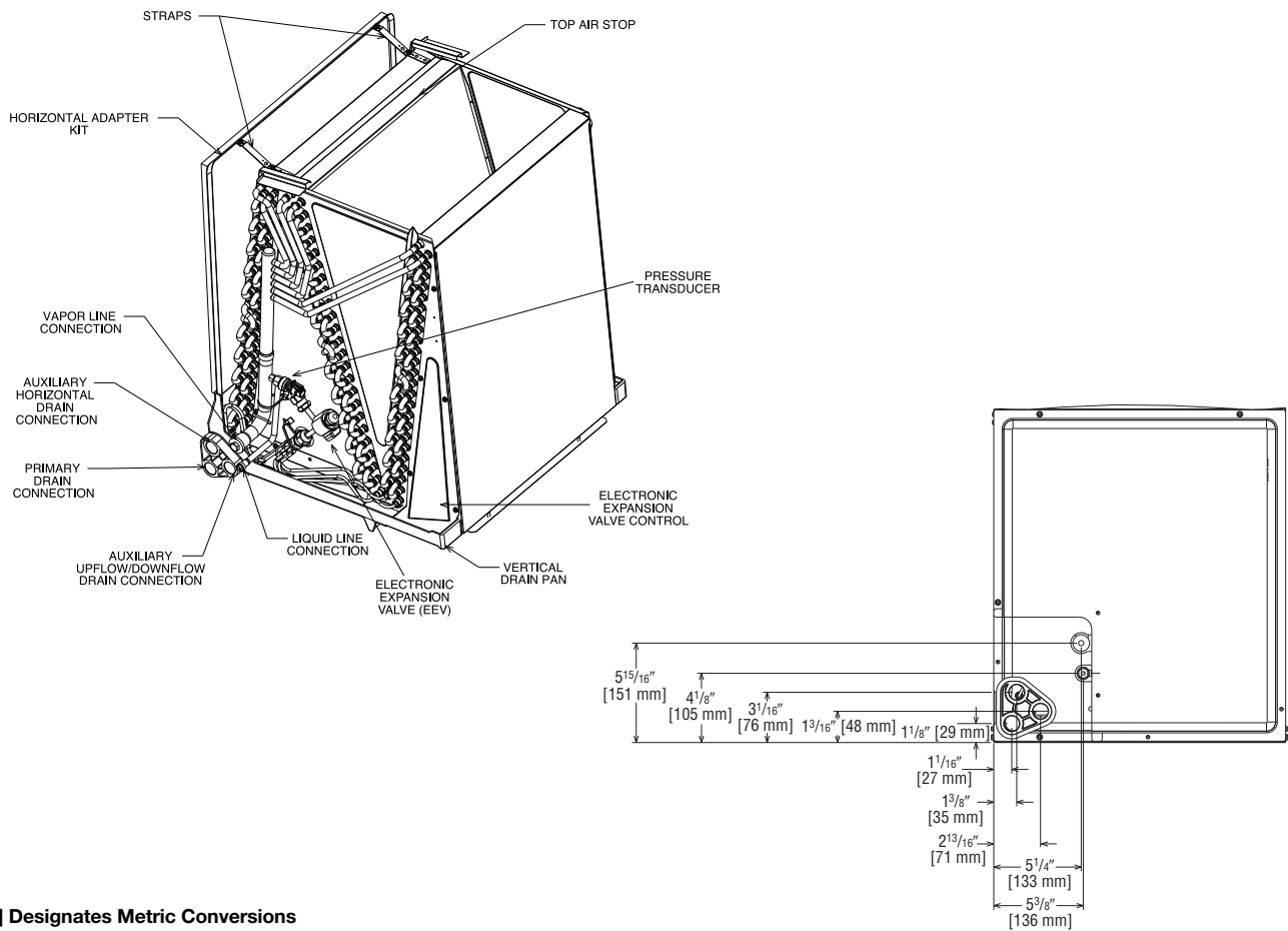
FIGURE 7 INDOOR COIL AND DRAIN PAN SET-UP
