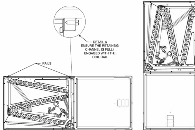
FIGURE 6 VERTICAL DOWNFLOW & HORIZONTAL RIGHT APPLICATION
