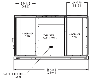
RIGHT DEDICATED VERTICAL AIRFLOW UNIT 181 SIZE
