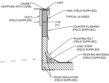
VIEW "B" CORNER DETAIL
