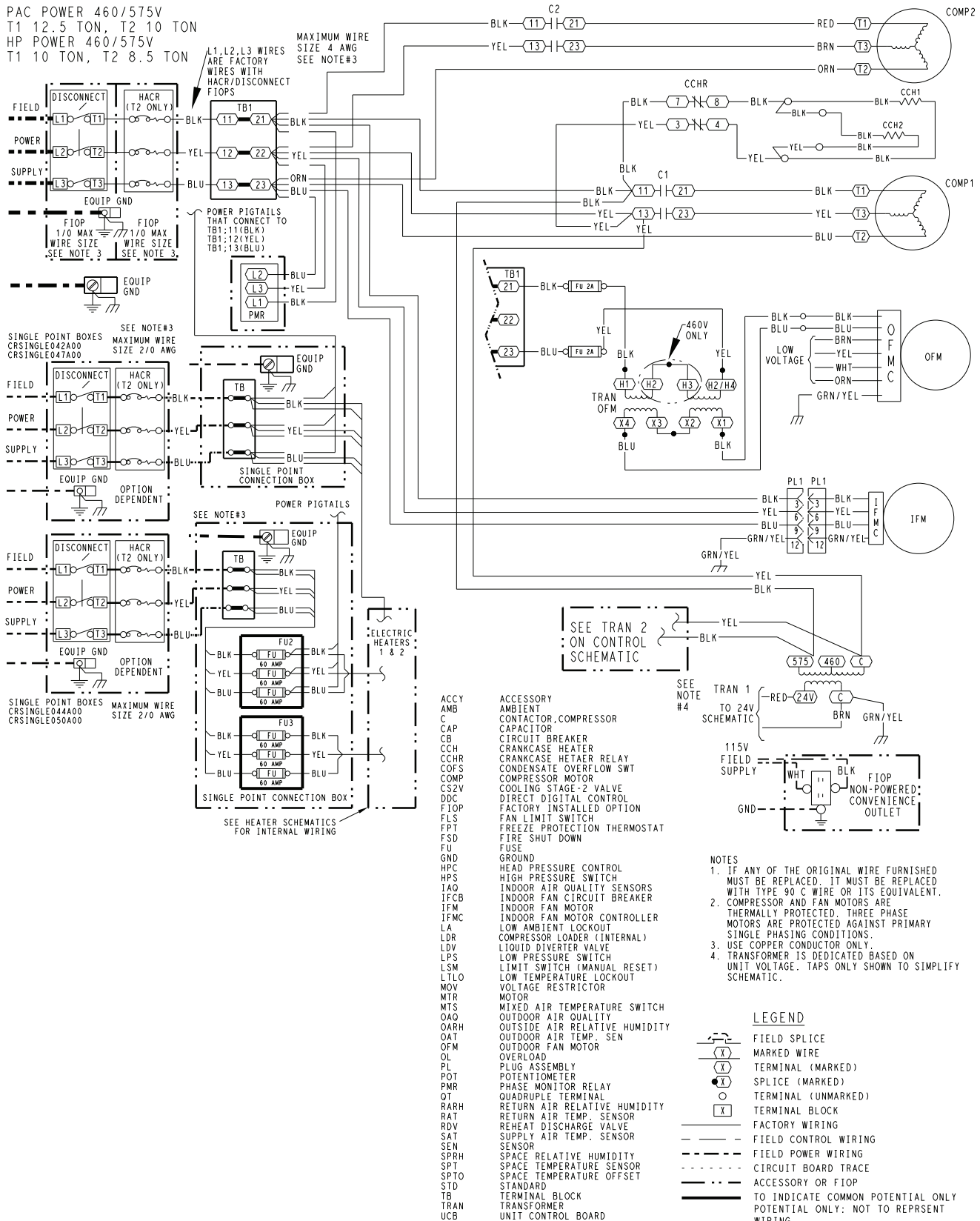
RHW102 Power Wiring Diagram, 460/575V-3-60 Shown
