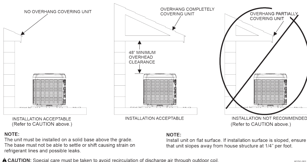
Figure 4: Typical installation
