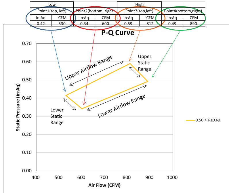
Figure 4. P-Q Curve Example
