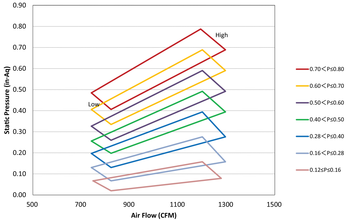
Figure 8. 4MUD4536A10N0A P-Q Curve Example
