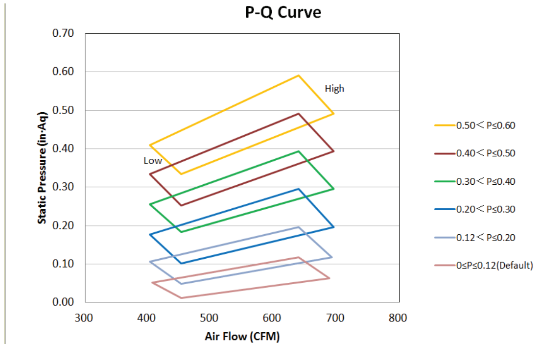
Figure 5. 4MUD4518A10N0A P-Q Curve Example
