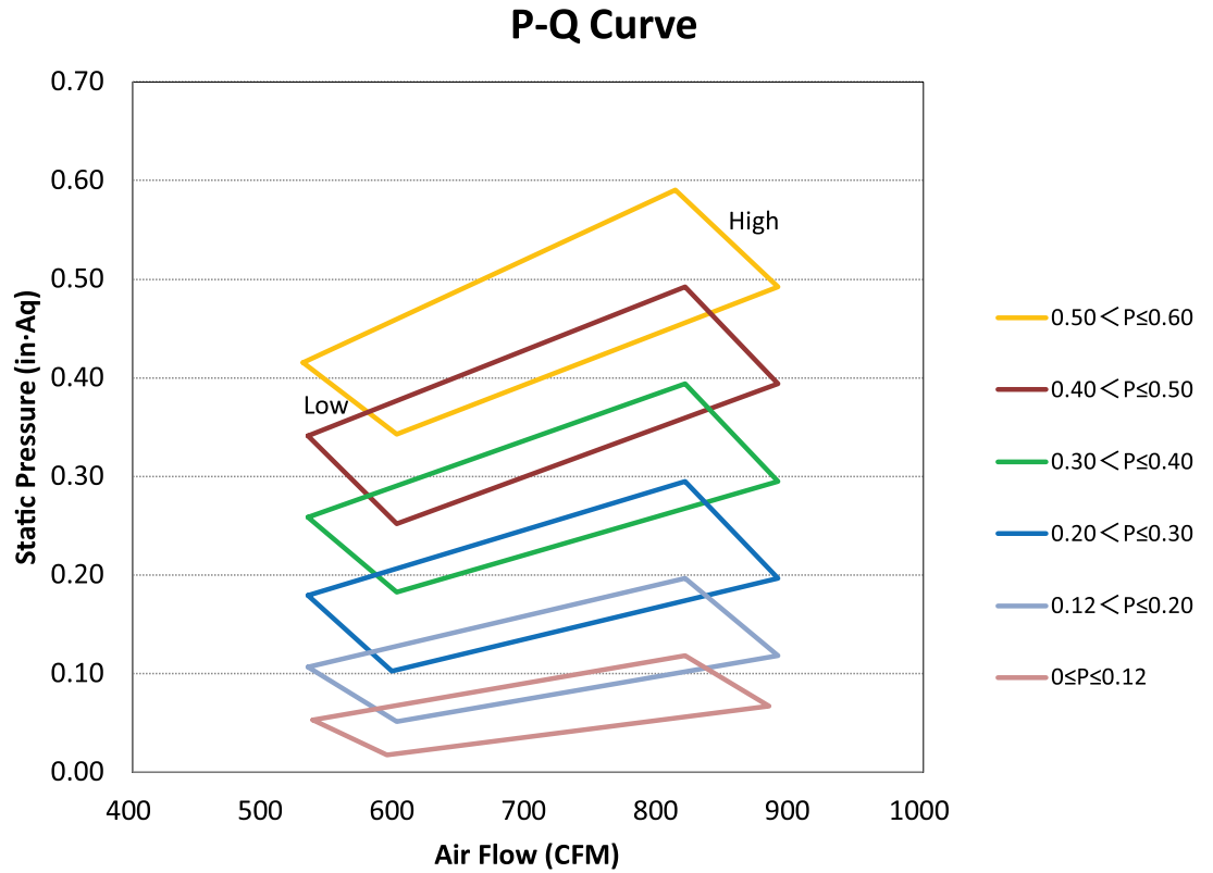
Figure 6. 4MUD4524A10N0A P-Q Curve Example
