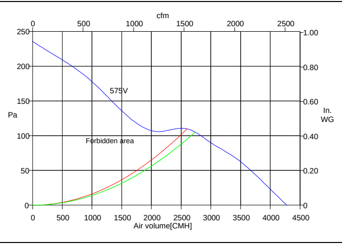
575-3-50 power exhaust fan curve
