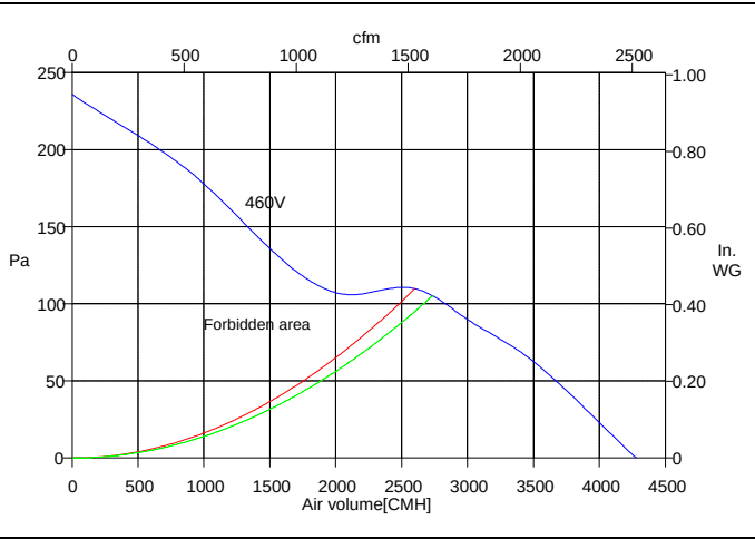
460-3-60 power exhaust fan curve
