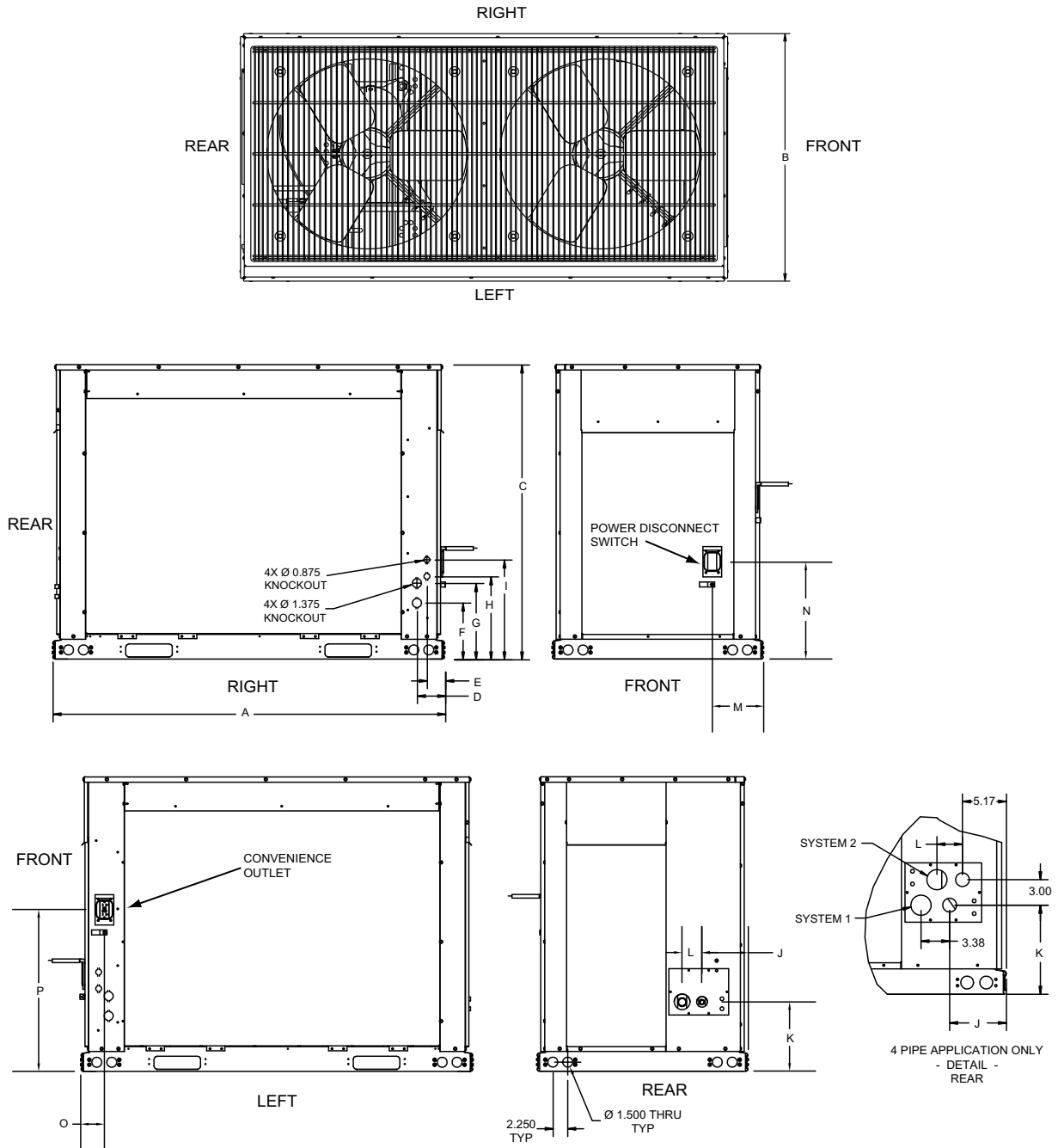
Unit Dimensions PC090, PC120, YC090, YC/YD120, YC/YD150
