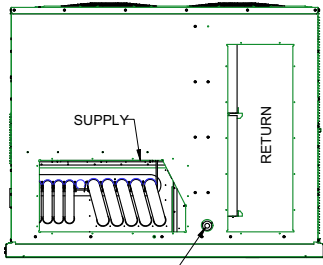
RIGHT VIEW
